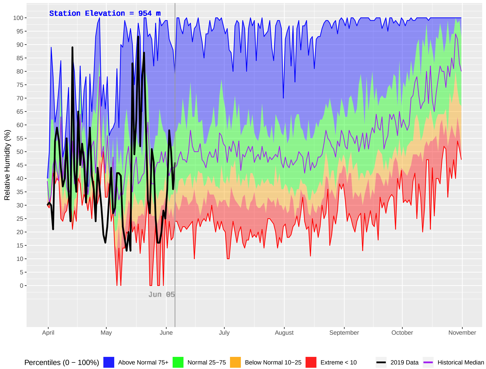
NADINA (179) : Historical (1985–2018) and Current (2019) Daily Relative Humidity
