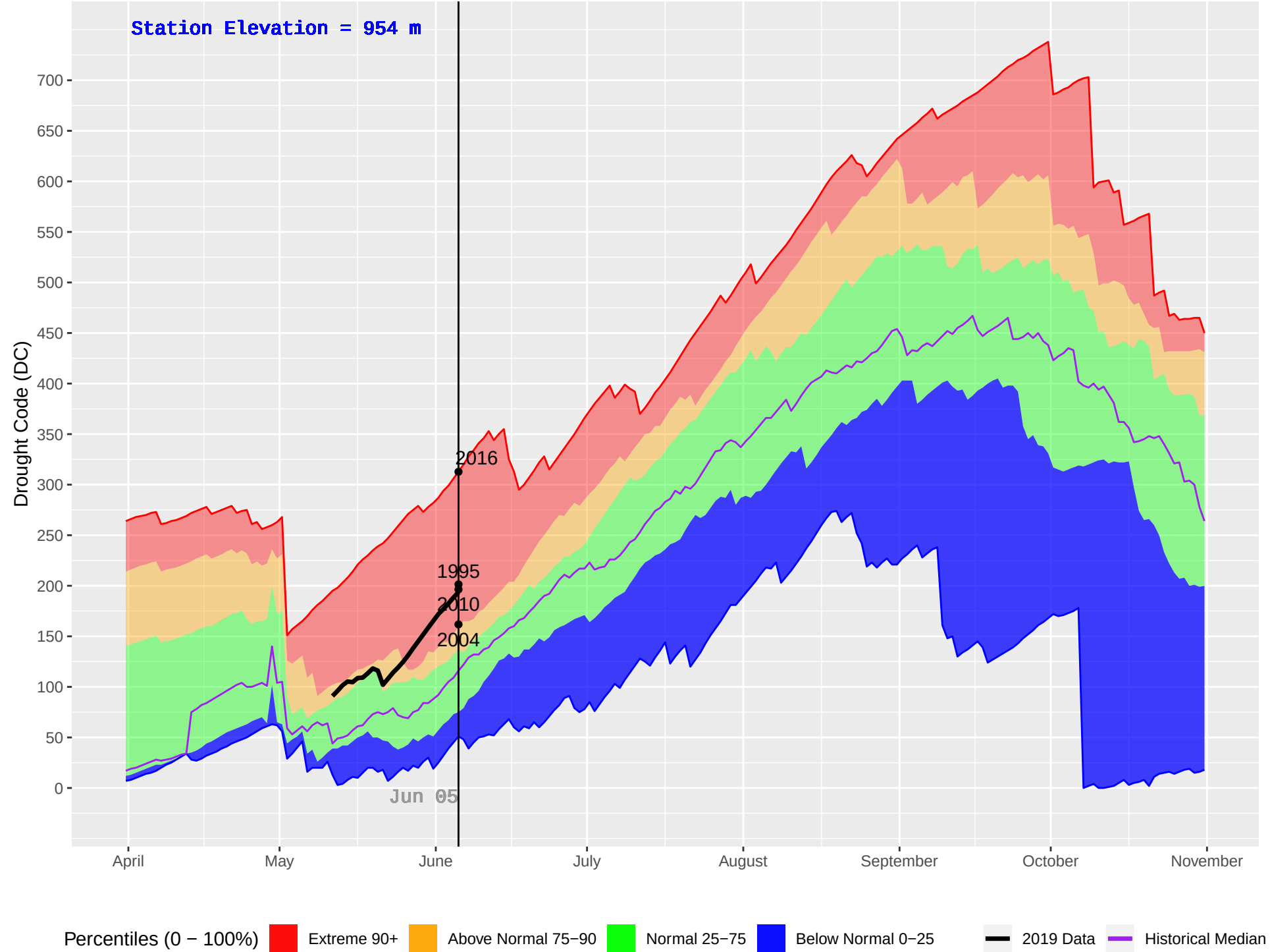
NADINA (179) : Historical (1985–2018) and Current (2019) Daily Drought Code (DC)
