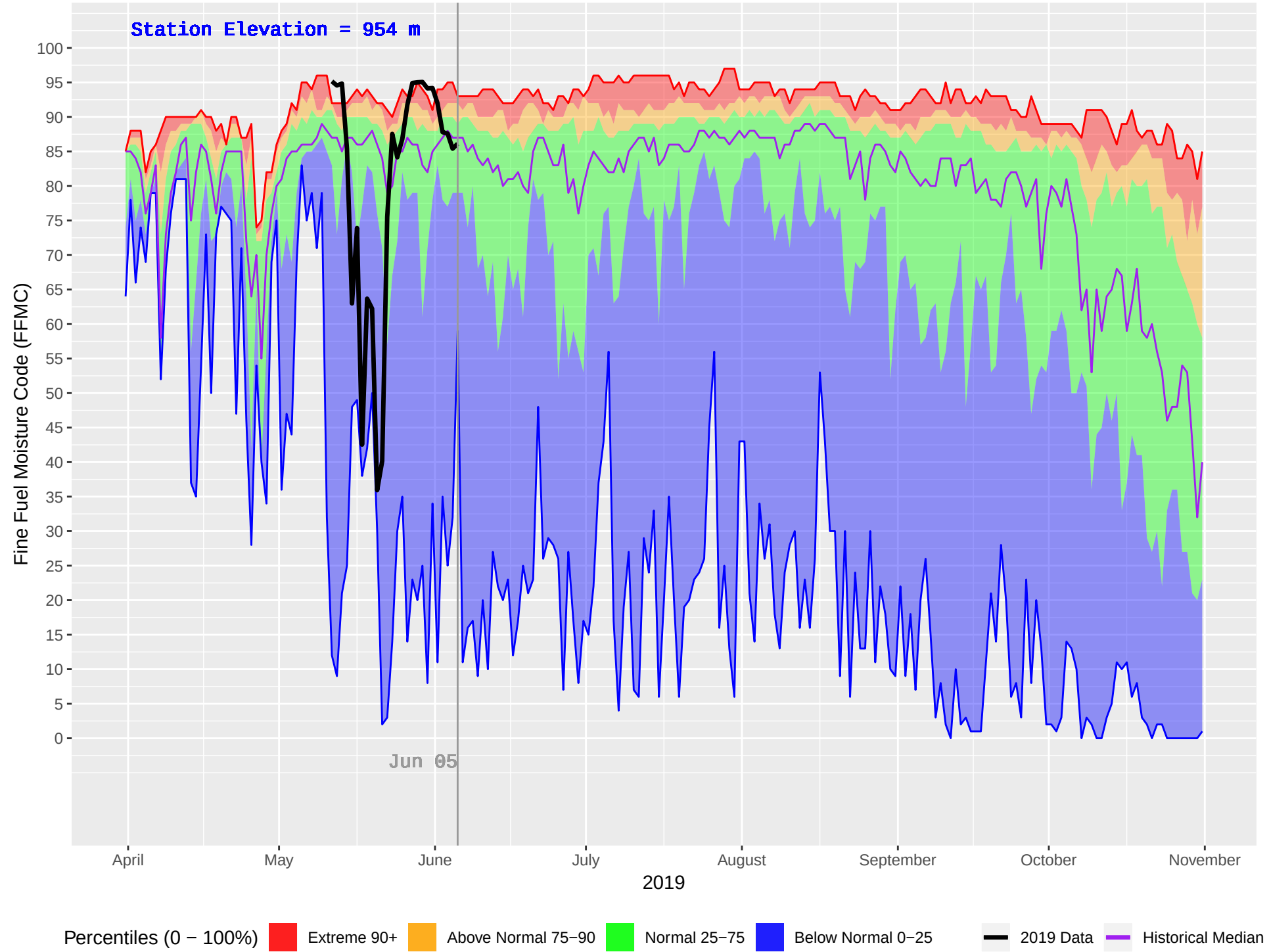
NADINA (179) : Historical (1985–2018) and Current (2019) Daily Fine Fuel Moisture Code (FFMC)
