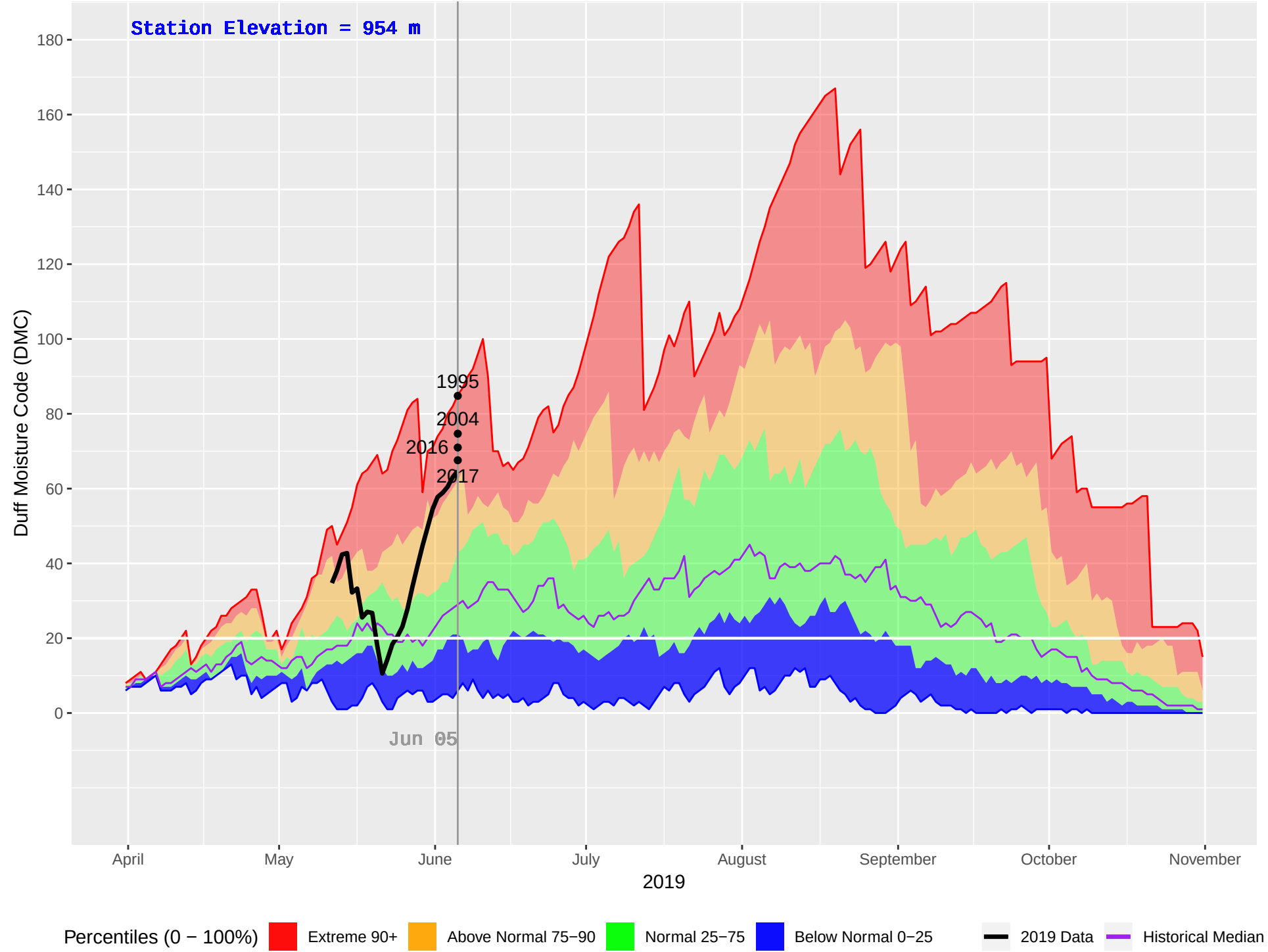
NADINA (179) : Historical (1985–2018), Current (2019) Daily Duff Moisture Code (DMC)
