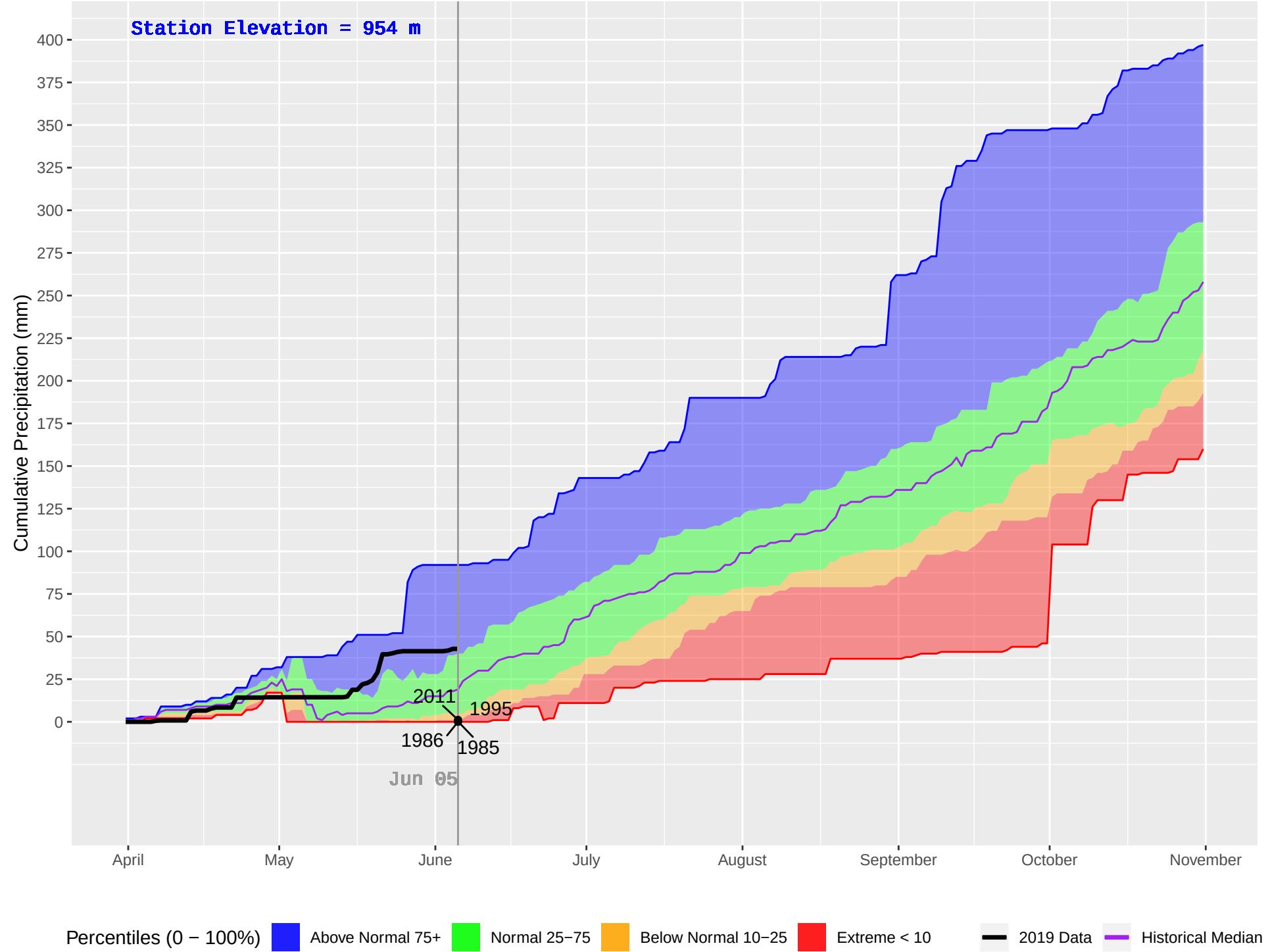
NADINA (179) : Historical (1985–2018), Current (2019) Daily Cumulative Precipitation
