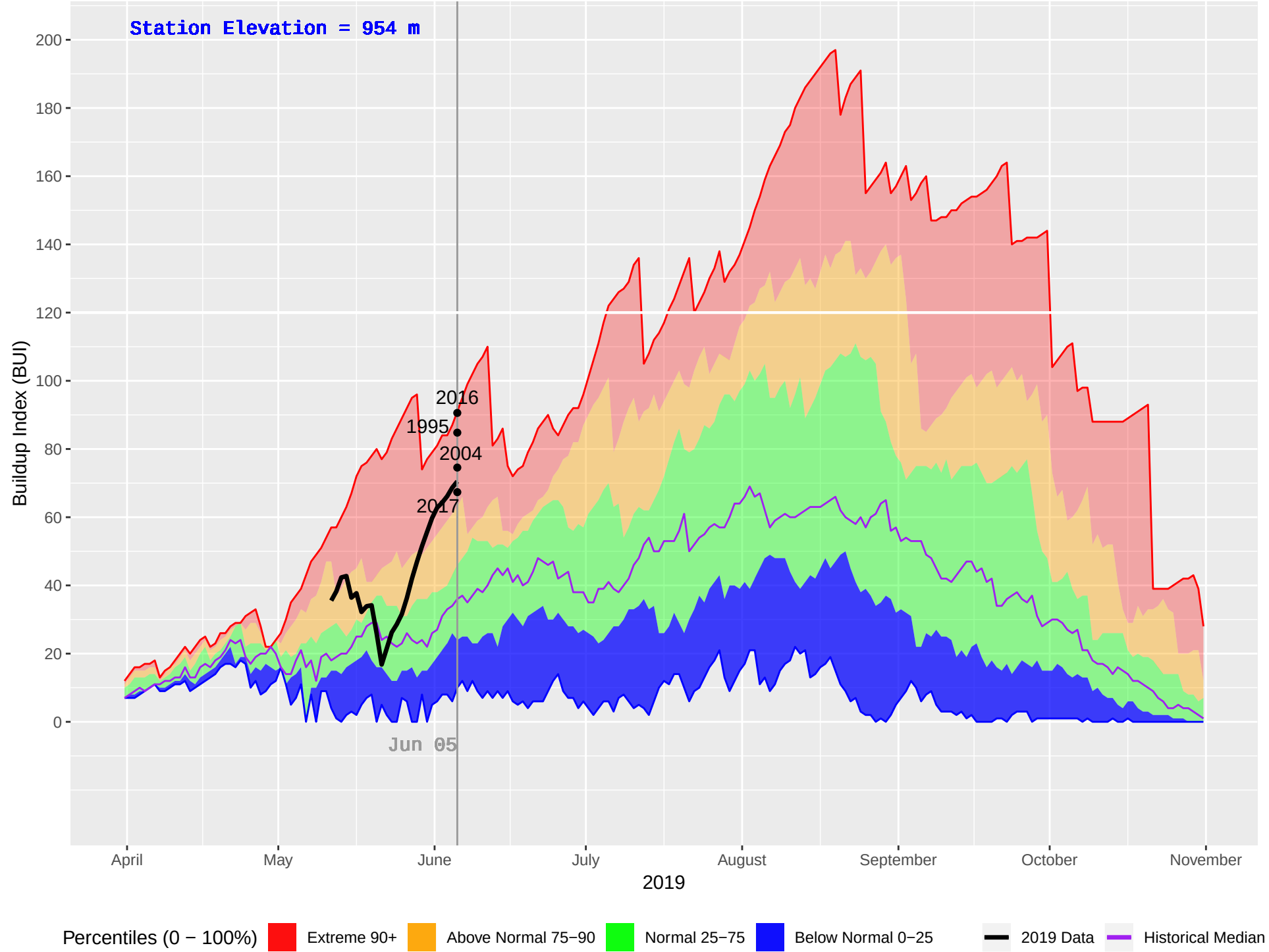
NADINA (179) : Historical (1985–2018), Current (2019) Daily Buildup Index (BUI)
